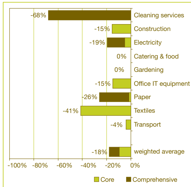
Figure 5.4: CO 2 impact of GPP in Finland. Negative numbers imply reductions in CO 2 emissions.
