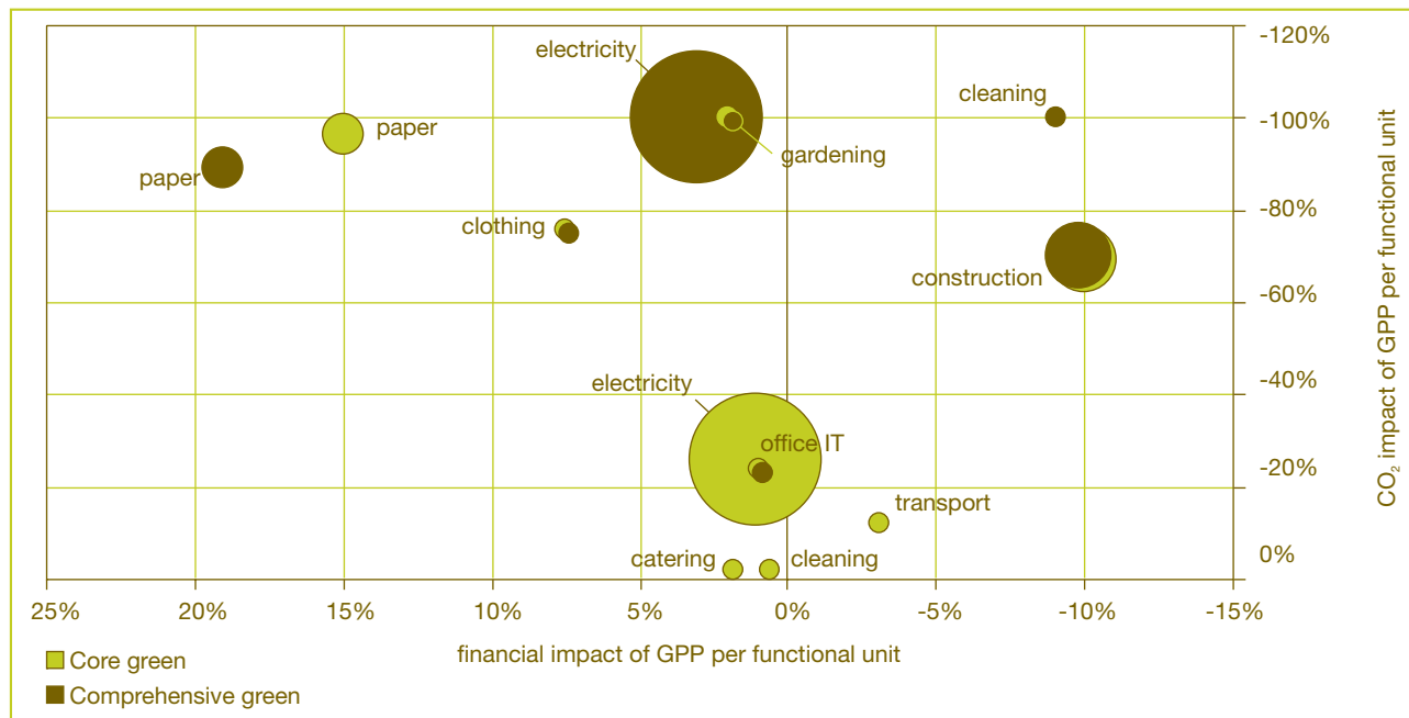
Figure 7: CO 2 impact and financial impact of GPP per functional unit. Negative numbers imply lower CO 2 emissions or lower costs and positive numbers imply higher costs.
