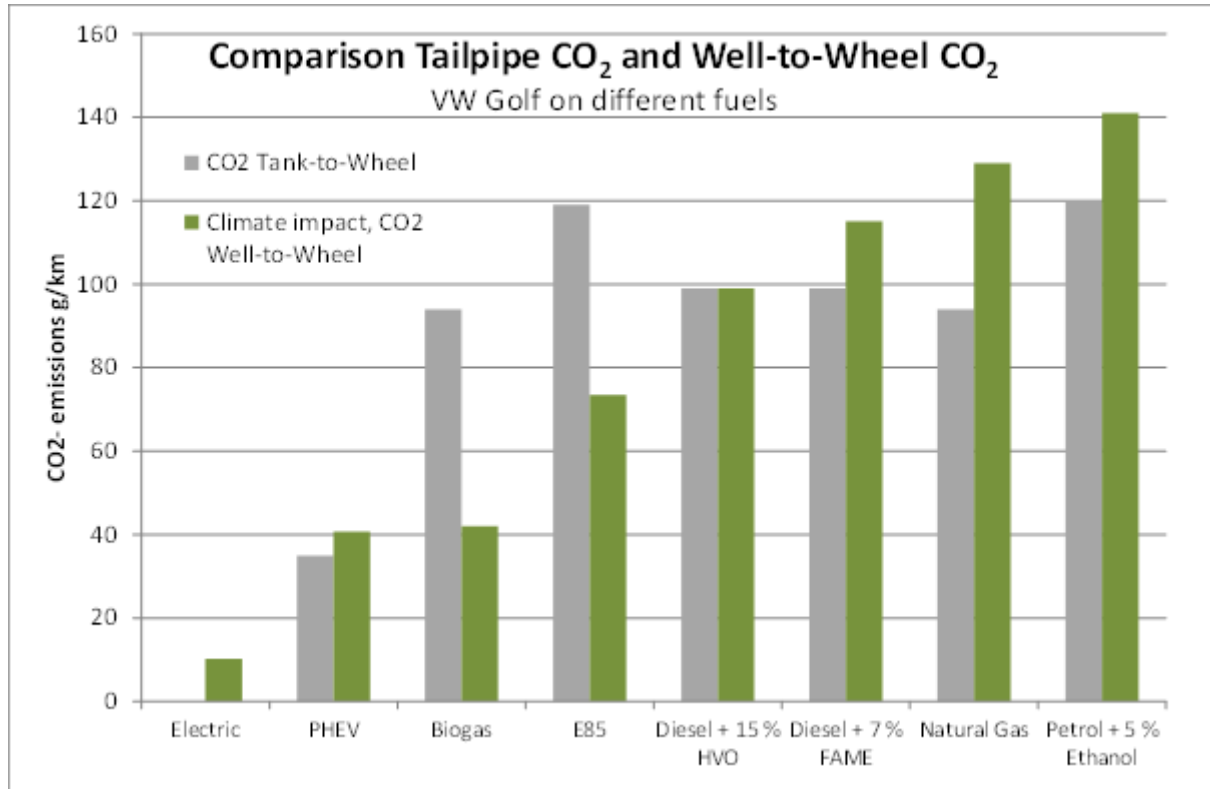
Fig. 1: Comparison between the Tailpipe CO 2 -value, shown in the vehicle register and the real climate impact CO 2 Well-to-Wheel, (based on Swedish biofuels sustainability values 2012)
